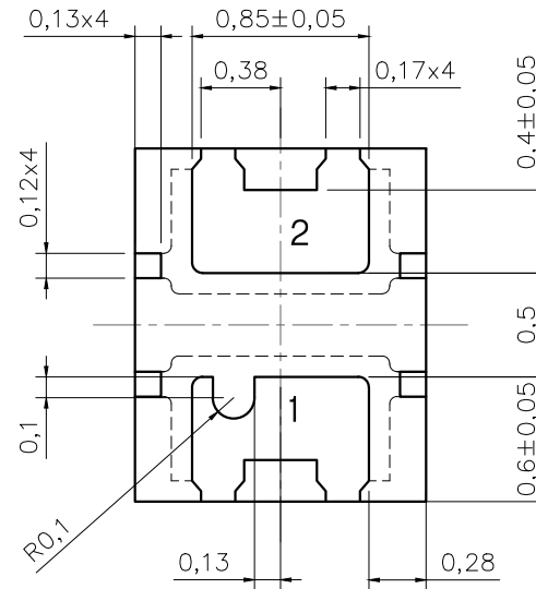
BOTTOM VIEW
